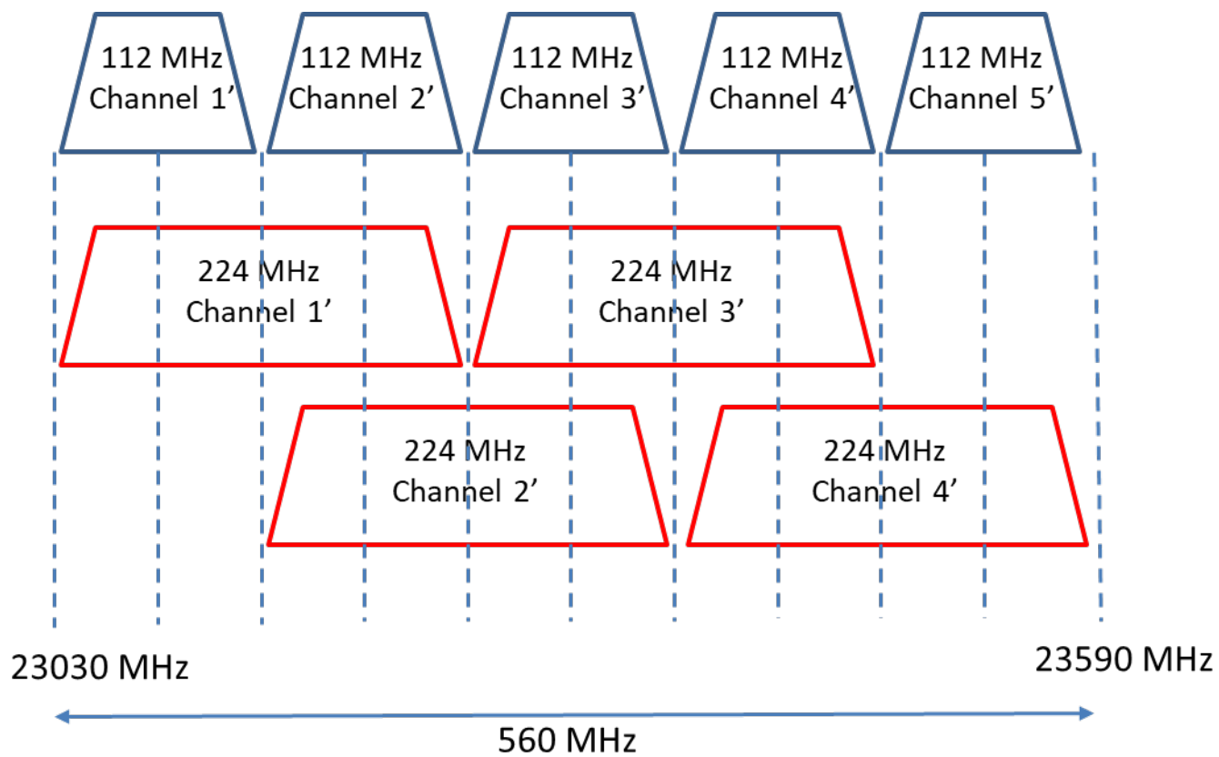
Figure 8: Channel arrangement and identifiers with channel width of 224 MHz (upper half of band)
